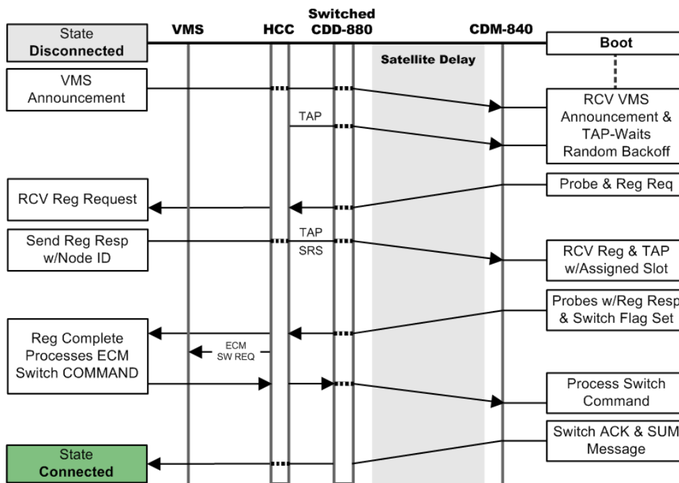
Figure F-1. ECM – Message Processing Diagram
