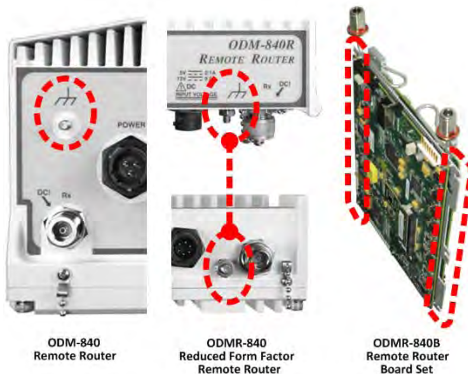
Figure 2-6. ODM-840 Chassis Ground Interface
