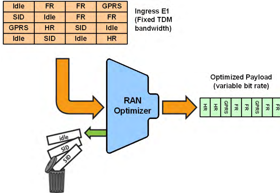
Figure J-3. RAN Optimization (GSM Abis Interface)
