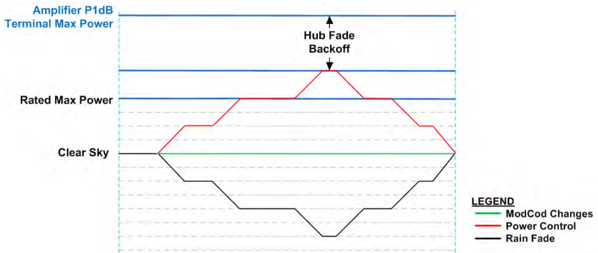
Figure L-7. DPC w/ACM with Hub Backoff
