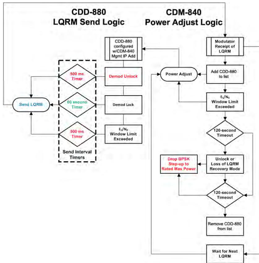
Figure L-4. LQRM / Power Management Flow Diagram
