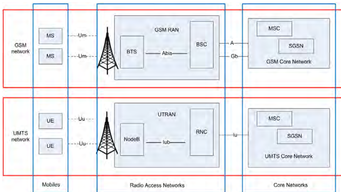
Figure J-1. 2G / 3G Radio Access Network (RAN)
