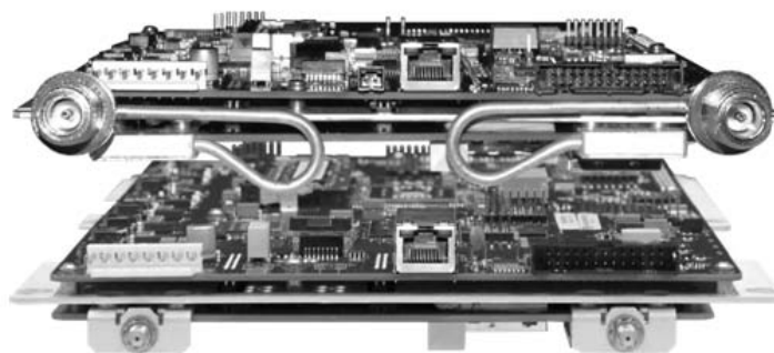
ODMR-840B Outdoor Remote Router Board Set (TOP) Type N Connectors Model (BOTTOM) Type SMA Connectors Model
