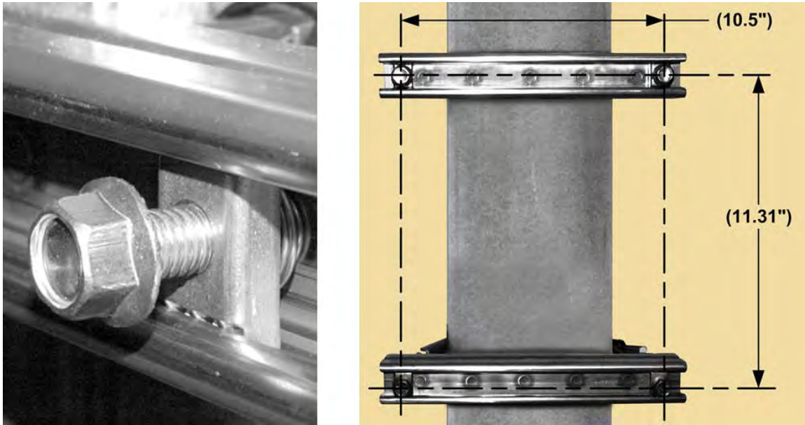
Figure 3-6. ODM-840 Unit Mounting – Spring Nut and Screw Installation and Spacing
