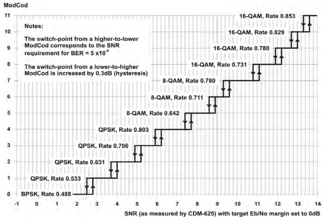
Figure D-4. ODM-840 – ACM ModCod Switch Points
