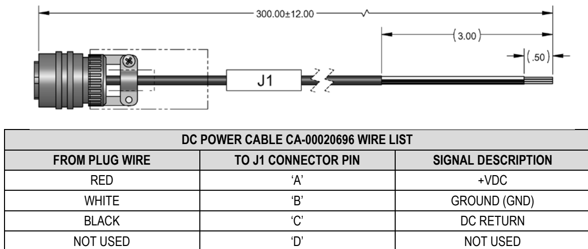
Figure 3-12. DC Power Cord (REF CEFD P/N CA-00020696)
