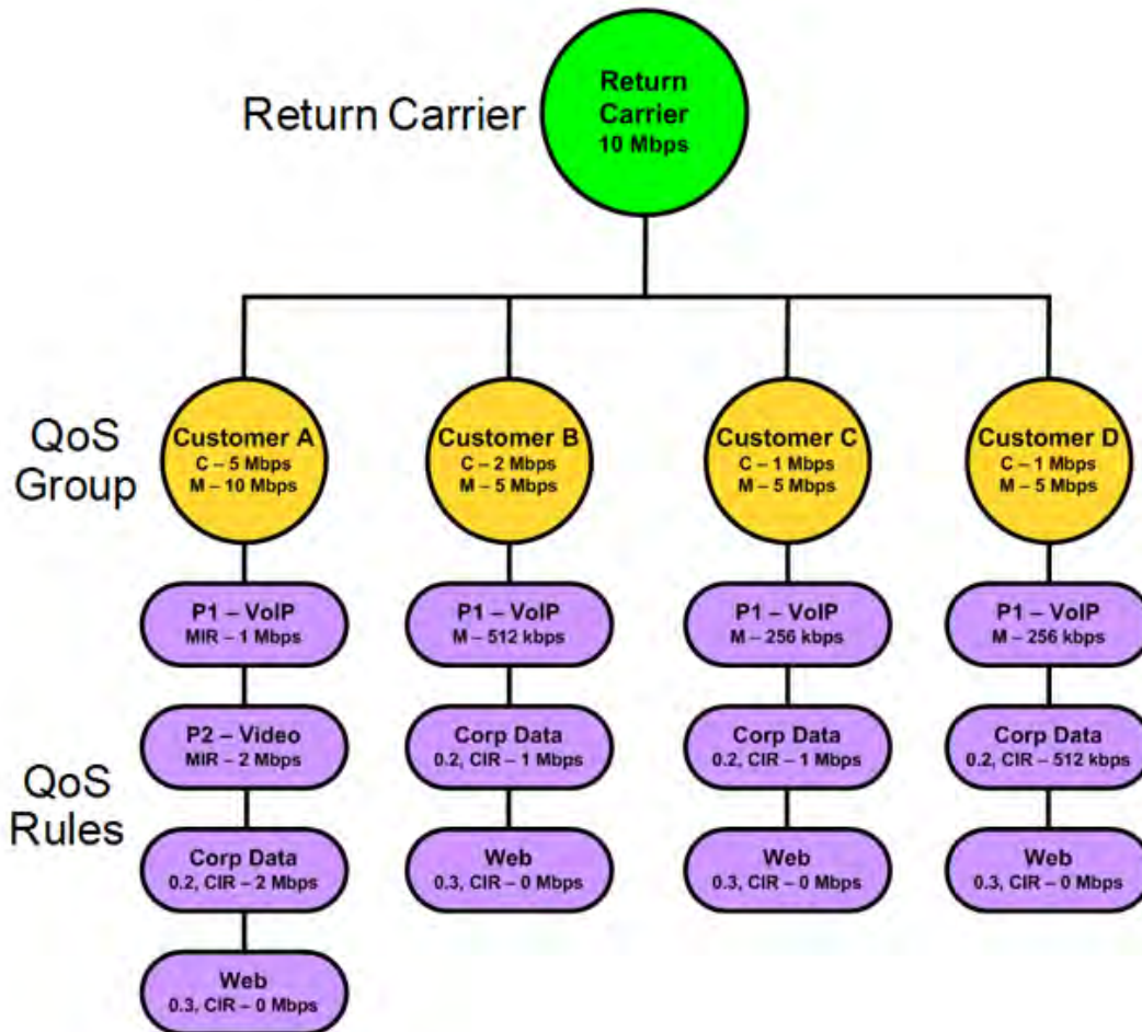
Figure H-2. Group QoS for Multi-tenant Site 2-Level Return QoS Configuration
