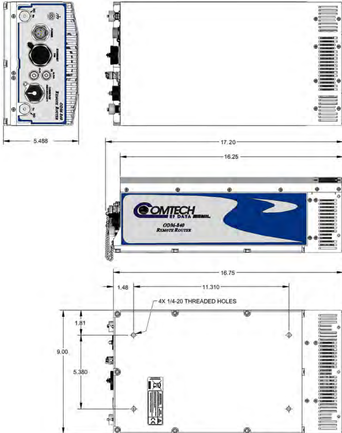
Figure 1-3. ODM-840 Dimensional Envelope
