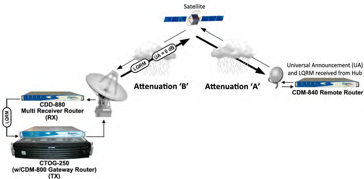
Figure L-6. Hub Rain Fade
