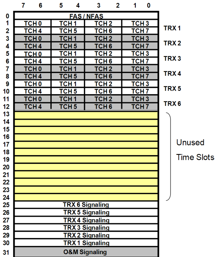
Figure J-2. Typical Abis Map
