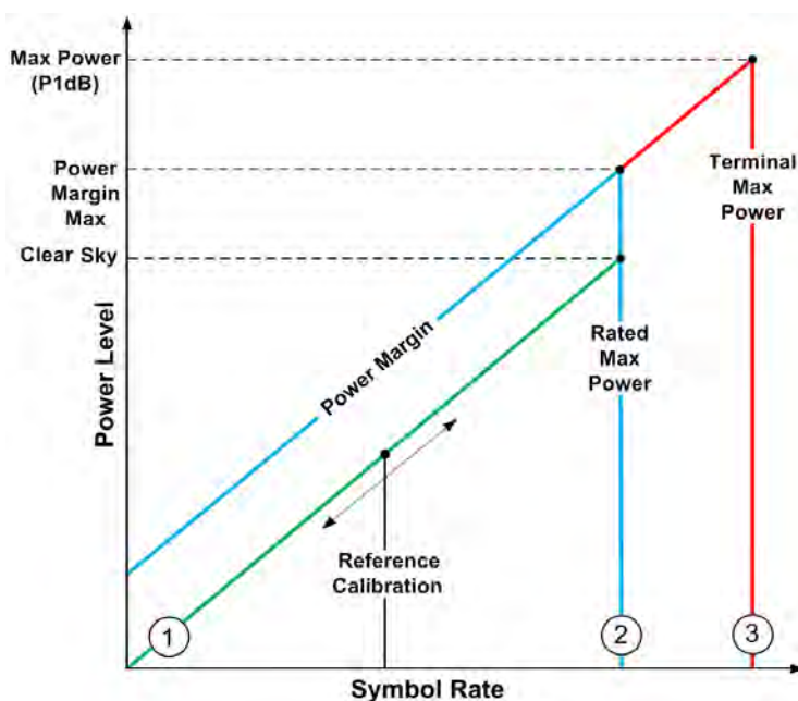
Figure L-1. DPC Power Scale
