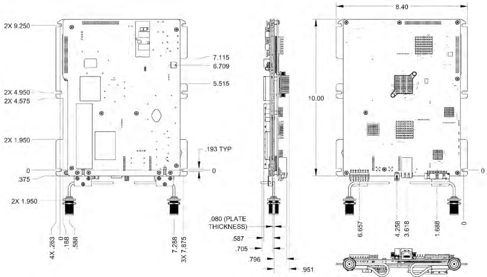
Figure 1-5. ODMR-8490B Board Set Dimensional Envelope – Type ‘N’ Connectors
