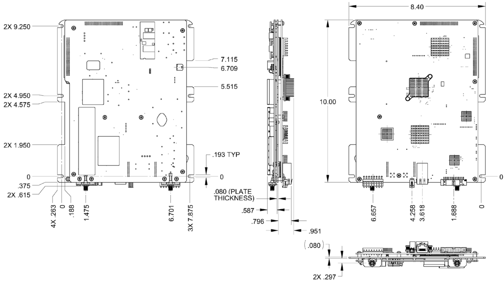
Figure 1-6. ODMR-8490B Board Set Dimensional Envelope – Type ‘SMA’ Connectors
