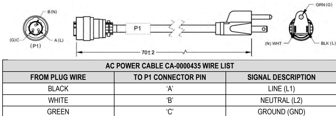
Figure 3-11. AC Power Cord (REF CEFD P/N CA-0000435)
