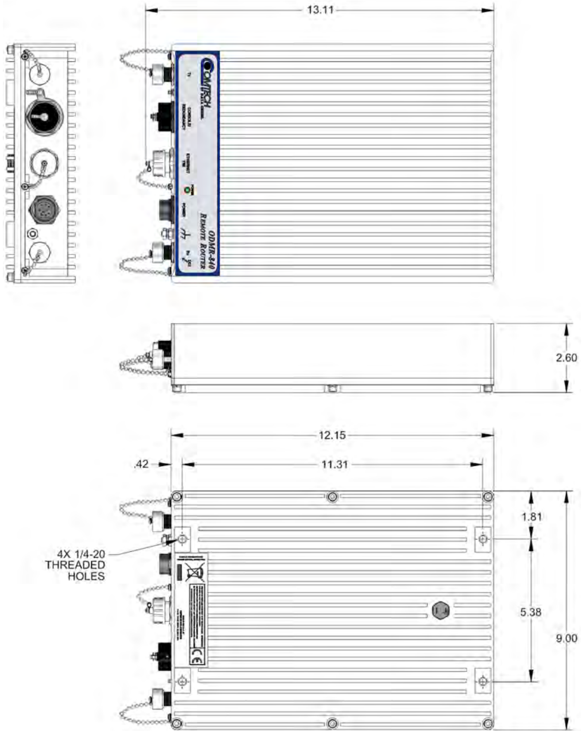
Figure 1-4. ODMR-840 Dimensional Envelope
